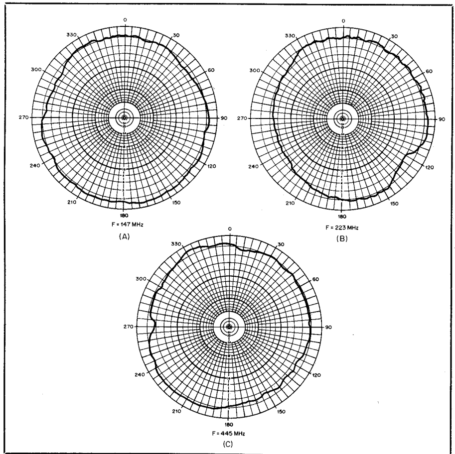
Fig. 3 — E-plane patterns for the three-band antenna. The patterns at A, B and C, respectively, are measured responses for 147, 223 and 445 MHz.
